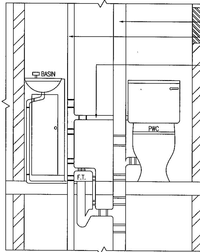
INSTALLATION OF PEDESTAL PAN AT WASH AREA Sketch Drawing 2
