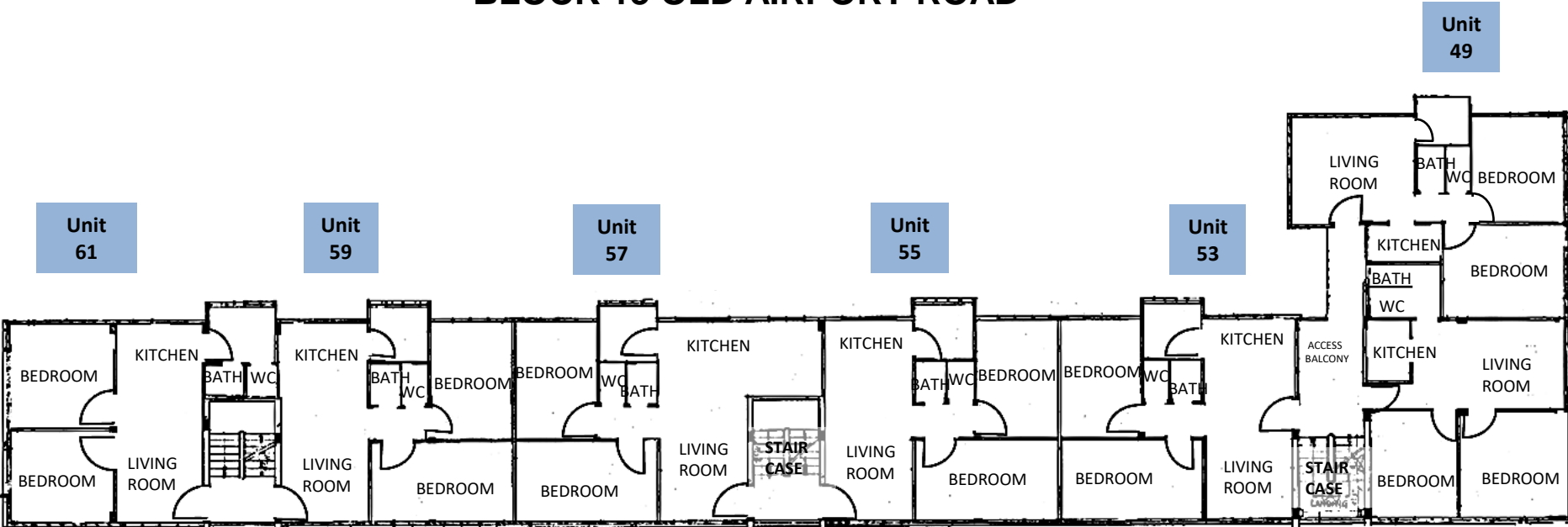
TYPICAL FLOOR PLAN AT 2 ND TO 3 RD STOREYS
