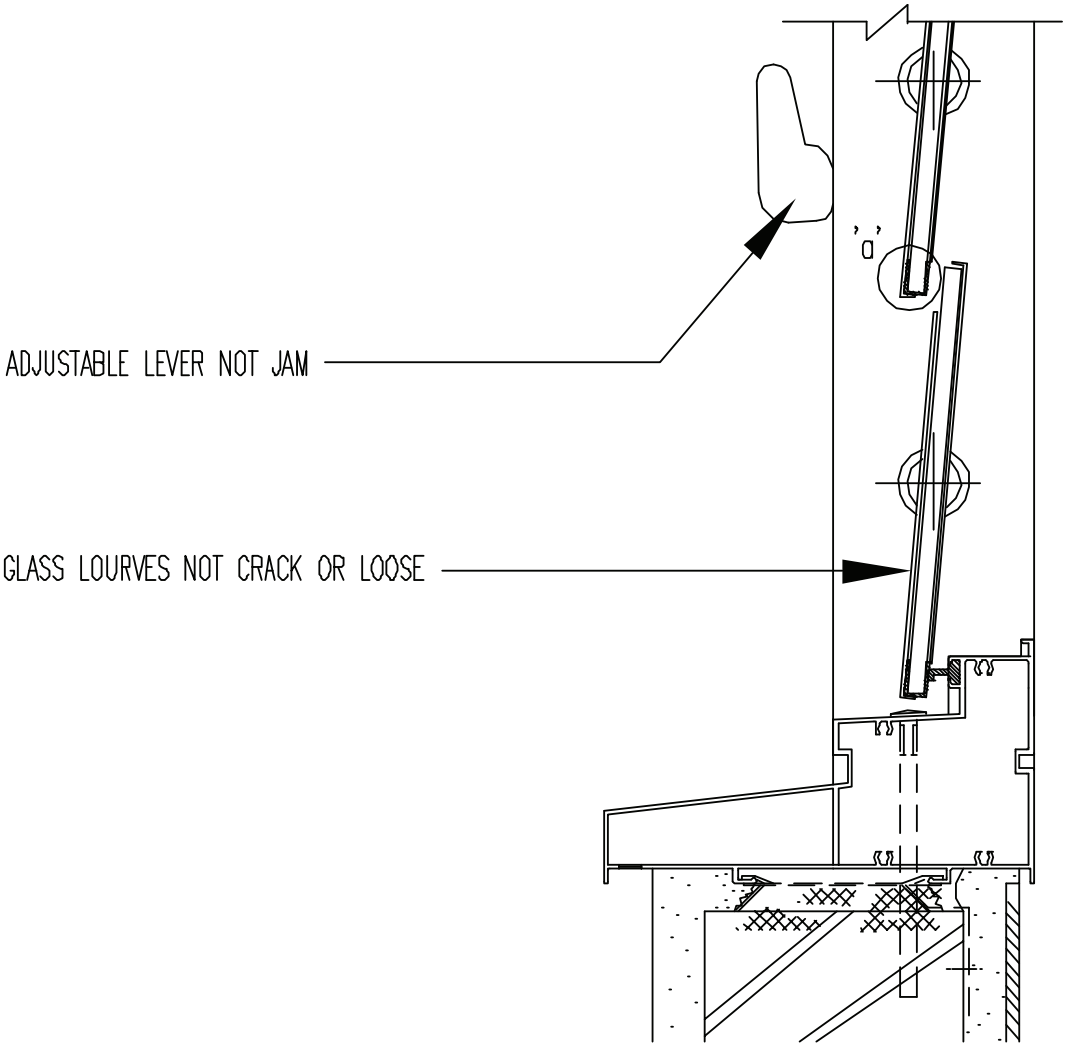
ADJUSTABLE ALUMINIUM LOUVRE VENTS
