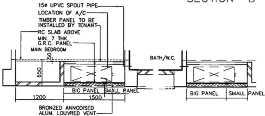
PLAN B
