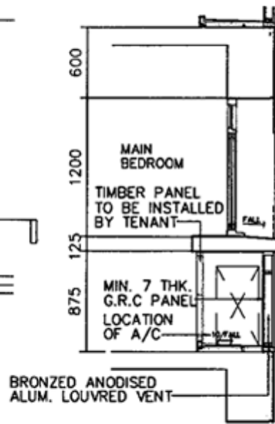
SECTION B-B
