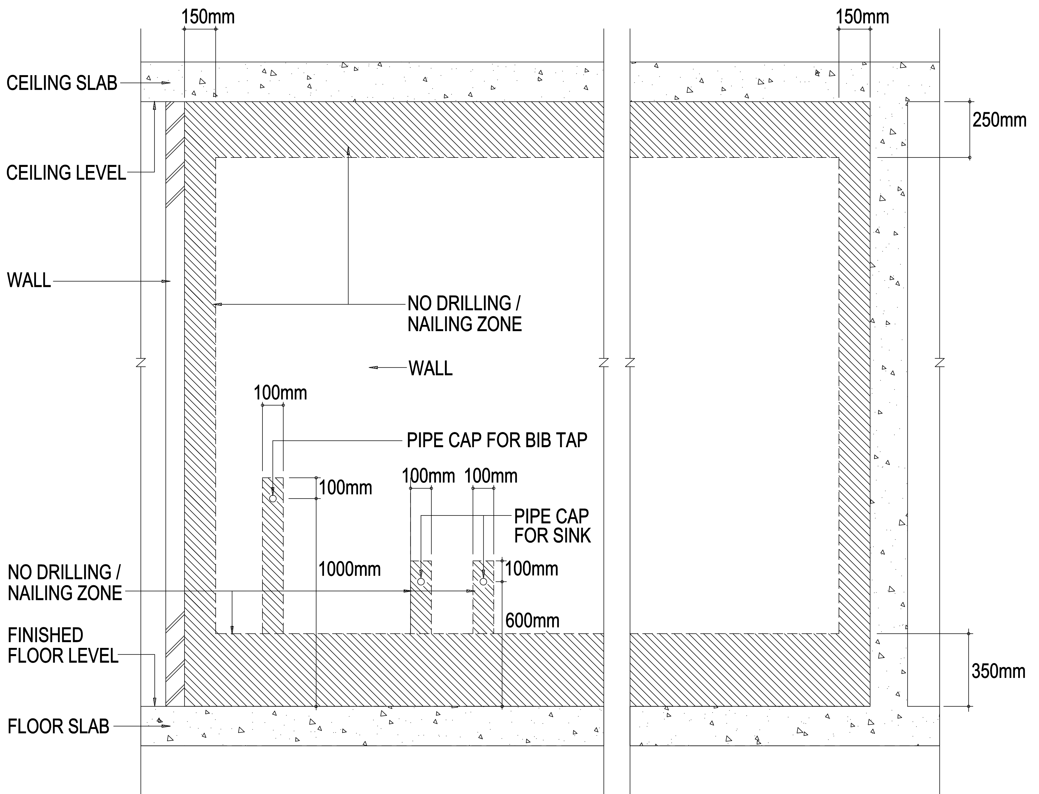
SECTIONAL VIEW
